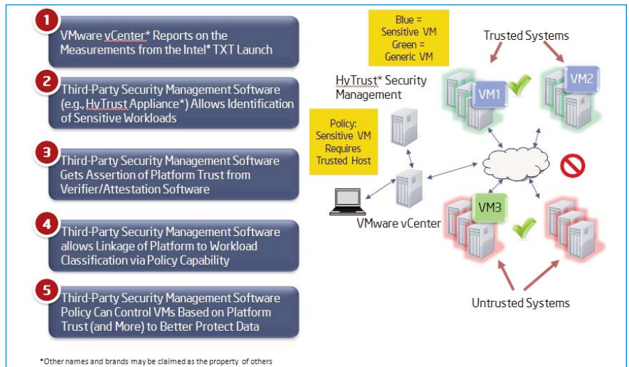
Figure 5. Creating the TCPs
